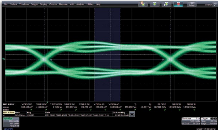
The eye diagram of an M-PHY signal illustrates portions of the eye that pertain to a specific measurement.
