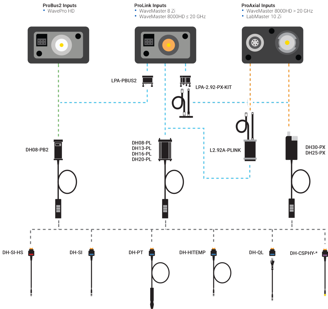
Differential High Bandwidth probe family
