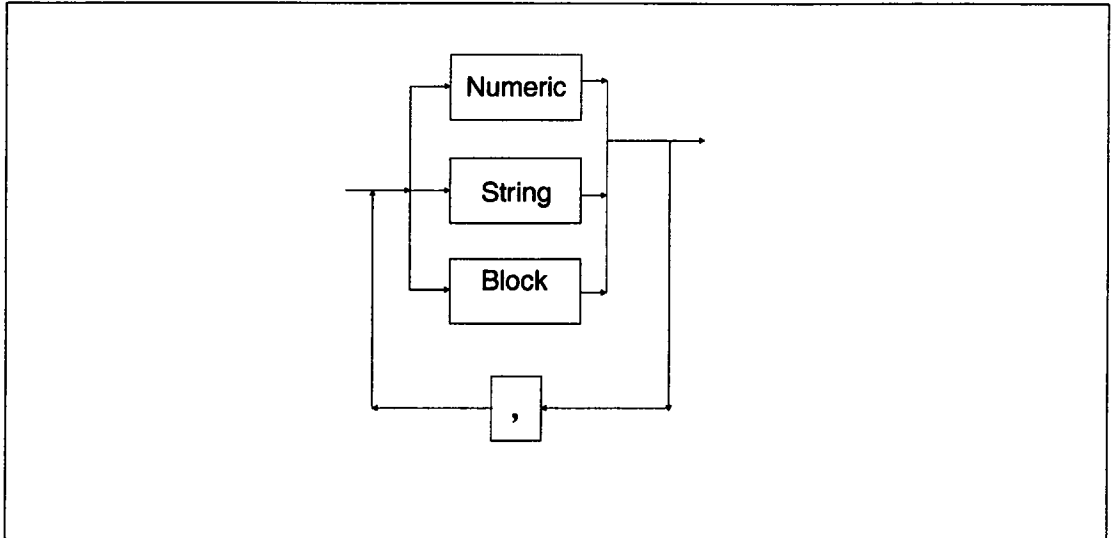
Figure 2.4: Command Arguments
