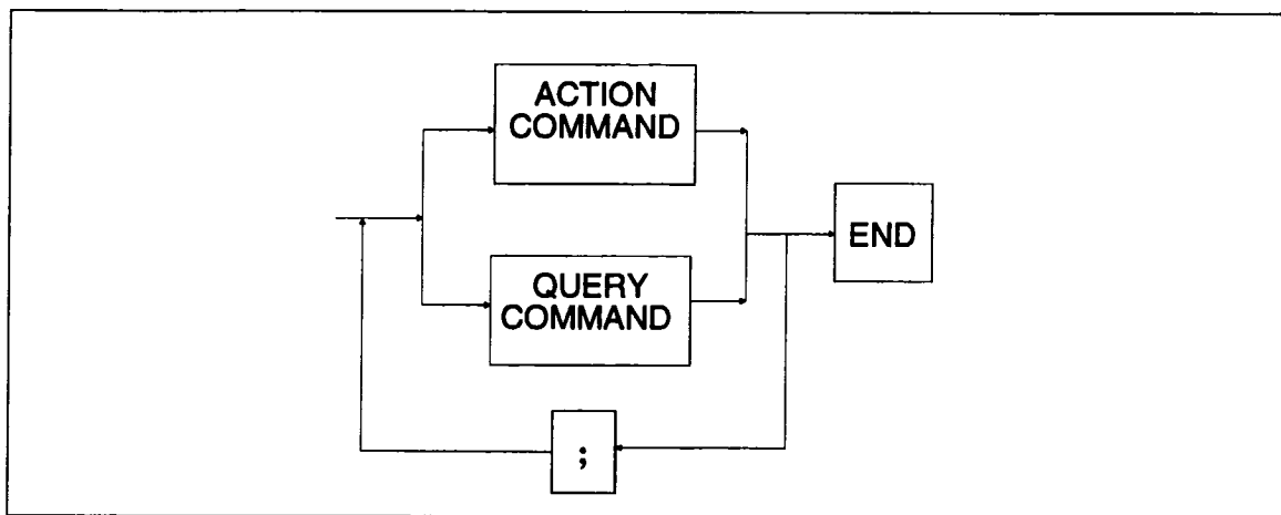
Figure 2.6: Multiple Commands
