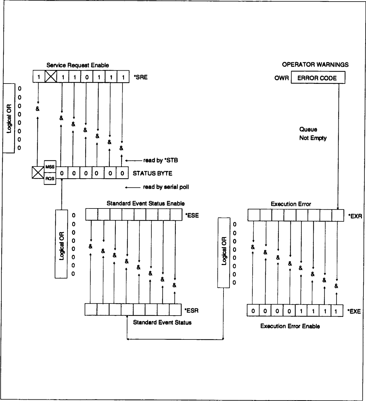
Figure 4.2 Event Enable
